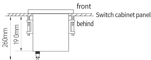
Installation diagram
