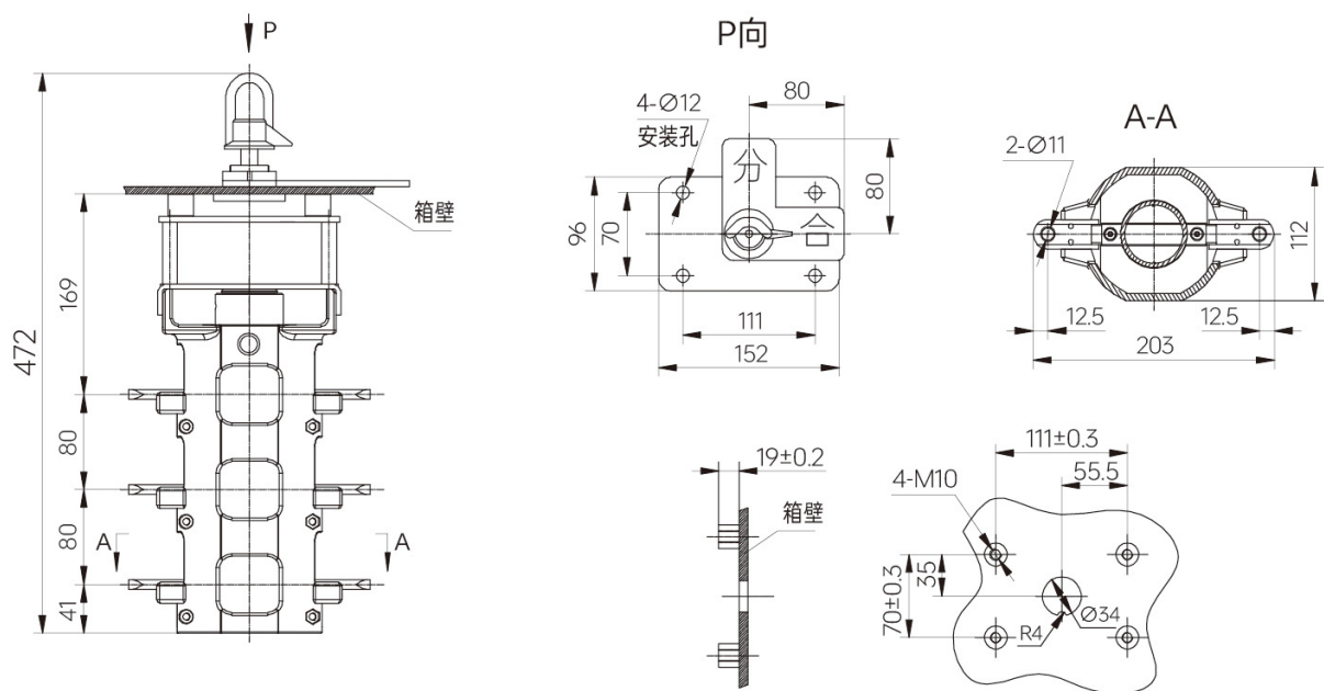
图1 ARF1-10/630 (315)-20-II
